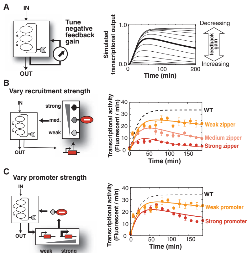
Fig. 3. Strength of synthetic negative-feedback circuit can be tuned by either altering recruitment affinity or inducible expression level of negative modulator. (A) Computational model (see supporting online text) predicts that adjustments in negative-feedback gain should tune adaptation behavior. (B) Adjusting feedback gain by varying modulator recruitment strength. Three affinity variants of the leucine zipper (strong, K_d = 6.1 nM; medium, K_d = 41 nM; and weak, K_d = 810 nM) were fused to Msg5 (negative modulator). Promoter controlling modulator expression was constant ( pPRM2 ). (C) Adjusting feedback gain by varying modulator promoter strength. Msg5-zipper is expressed from two mating-induced promoters: strong, pFIG1 , and weak, pPRM2 (fig. S4). Zipper fused to Msg5 was constant (weak). Orange plots in (B) and (C) show same strain (circuit with weak zipper and weak promoter). Points represent mean values for three experiments \pm standard deviation.
